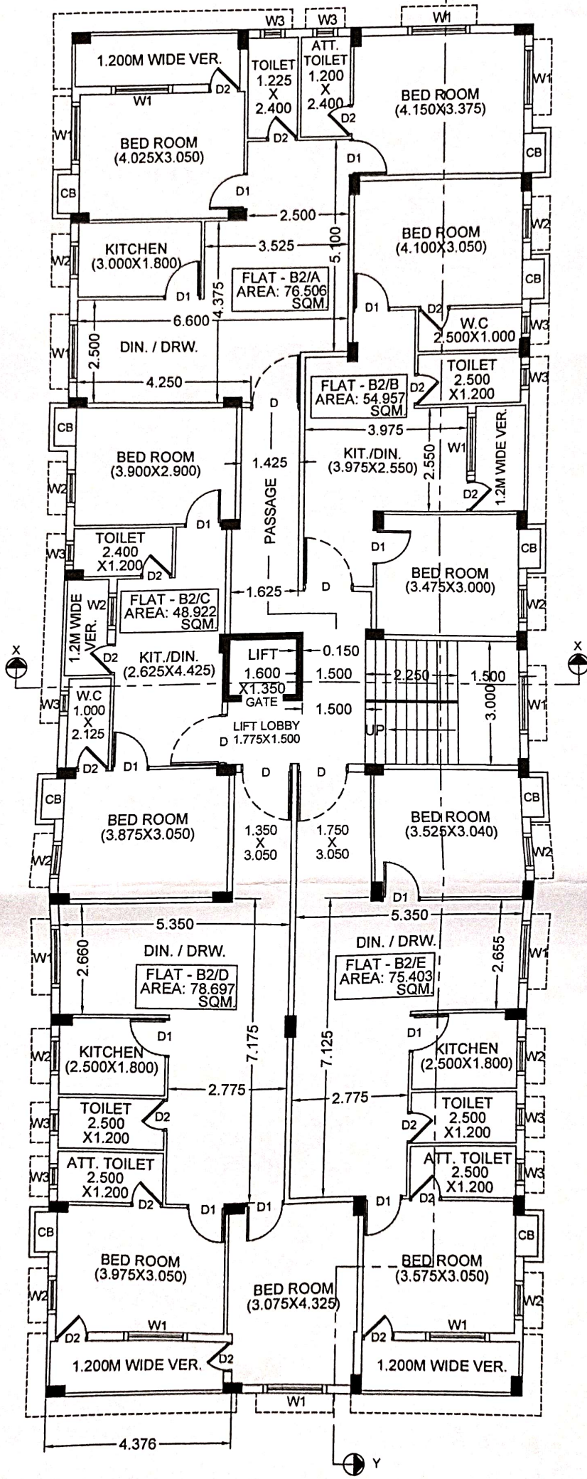
PROPOSED TYPICAL FLOOR PLAN OF BLOCK-2 (SCALE - 1:100)
